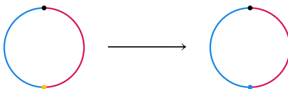
FIGURE 1 A nonconical stratification of S^1 is pictured on the right. On the left is a conical refinement of the right-hand stratification.
